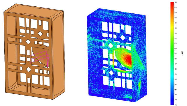
Fig. 1. Single-offset reflector antenna inside 6U CubeSat chassis (the front and back panels have been removed to give a better view of the antenna). Left: Reflector and open CubeSat chassis. Right: Simulated MoM currents on reflector and opened CubeSat chassis at 86 GHz.
