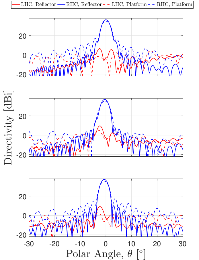
Fig. 3. Directivity patterns. [Blue/red] curves are [RHC/LHC], [solid/dashed] curves are for the reflector [alone/mounted in platform]. The top panel shows pattern cuts in the \phi = 0^\circ cut, the centre shows the \phi = 45^\circ cut, and the bottom shows the \phi = 90^\circ cut.
